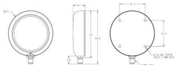
Dimensions (mm)
